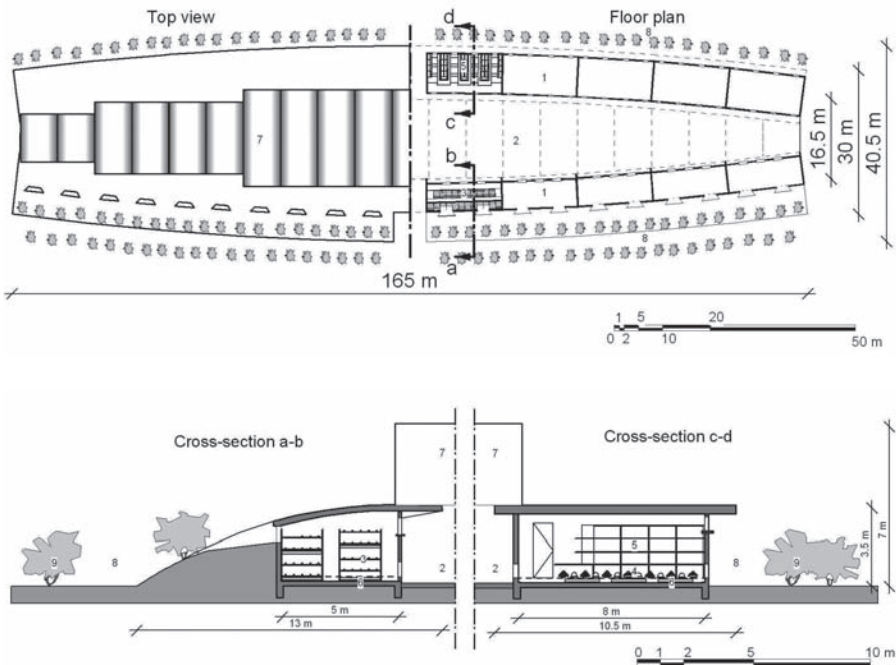
Figure 6. Plantation design. Top view, floor plan and cross-sections of the two houses of one unit. 1: unit for 3000 hens; 2: inner foraging area; 3: perches (for resting) over manure belts; 4: water and feed supply; 5: laying nests; 6: manure belts at floor level; 7: roof of semicircles covered with plastic foil that can be opened and closed; 8 and 9: outer area with shrubs & trees. (drawn by JvR Architectuur)
