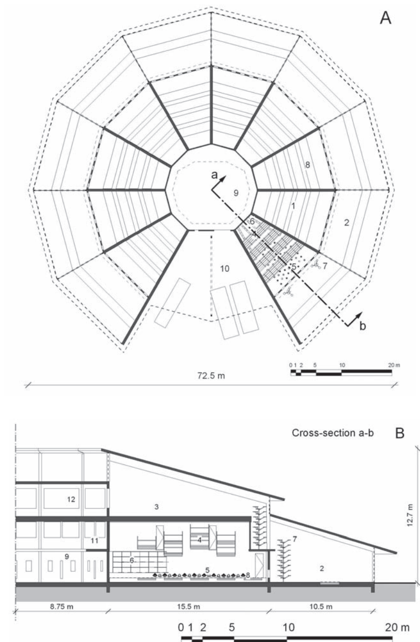
Figure 5. Roundel design. Top view (A) and cross-section a-b of one segment (B). 1: unit for 3000 hens; 2 & 3: foraging areas; 4: perches (for resting) over manure belts; 5: water and feed supply; 6: laying nests; 7: artificial trees; 8: manure belts at floor level; 9: room for collecting eggs; 10: expedition; 11: visitors and control gallery; 12: technical installations. (drawn by JvR Architectuur)
